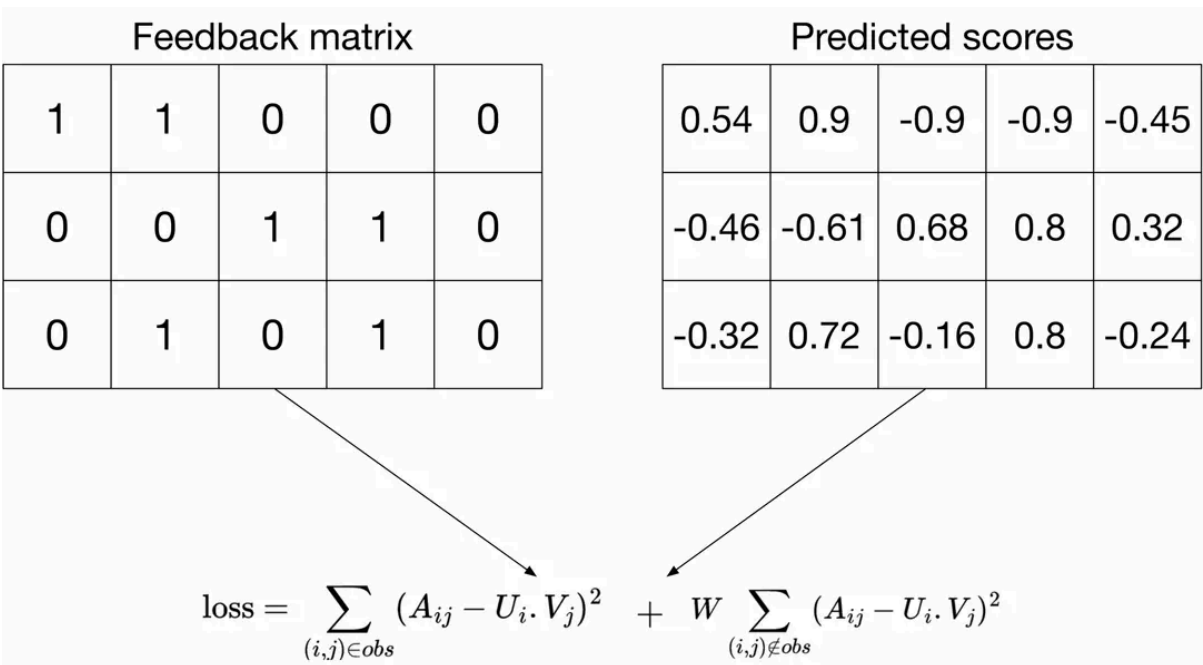
Figure 6.16: Combined loss
