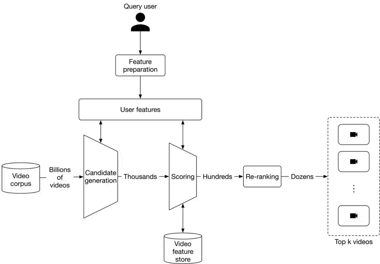
Figure 6.23: Prediction pipeline
