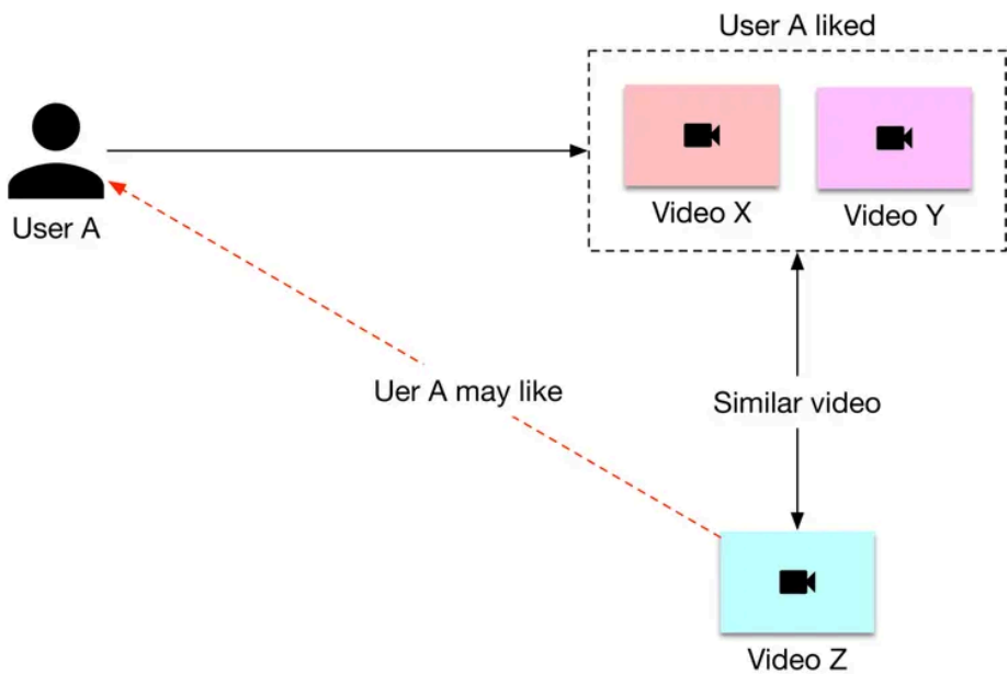
Figure 6.4: Content-based filtering
